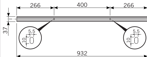
ROTATING LED TUBE
